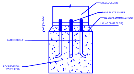
SAMPLE DETAILS OF MINIMUM PEDESTAL REQ. FOR PINNED BASE FOR ALL LEAN-TO COLUMN
